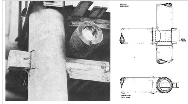
Gambar 5. Plugin/Bolt Connection (Katarzyna, 2013)
