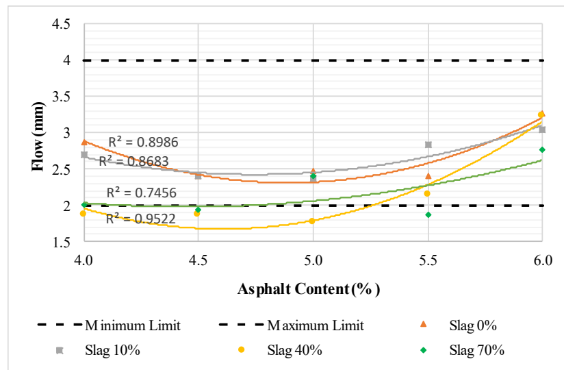
Figure 8. Flow vs Asphalt Content
