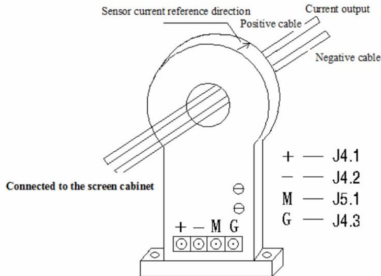
Figure 7. Hall CT design for leakage current detector (ground fault)
