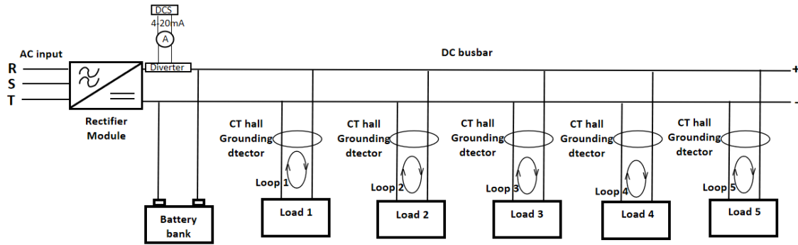
Figure 8. Closed loop in each branch load
