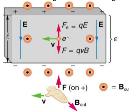
Figure 3. Description of the Lorentz force in the hall effect phenomenon (B) direction of the magnetic field approaching the screen (F) direction of the Lorentz Force (v) speed in the direction of the electric flow (l) width of the conductor plate (E) potential difference due to the hall effect.
