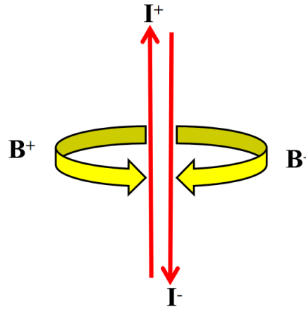
Figure 6. Overview of the direction of electric current and magnetic field in positive (+) and negative (-) cables
