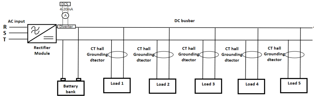
Figure 2. Diverter installation in the DC system
