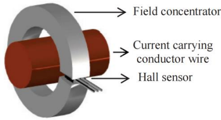
Figure 4. Design of magnetic field concentrator
