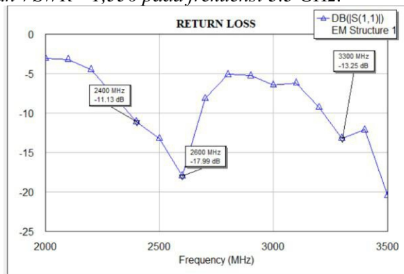
Gambar 4.1 Return Loss
