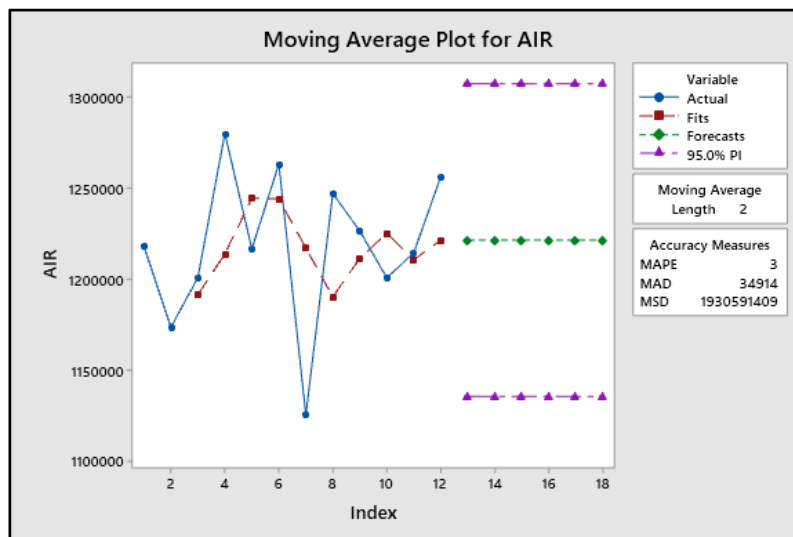
Figure 3. Forecasting using the moving average method
