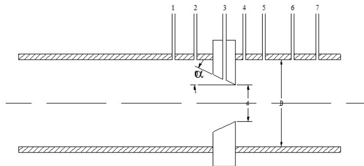
Gambar 4. Posisi pressure tap
