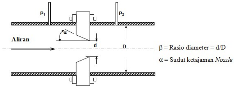
Gambar 3. Nozzle section
