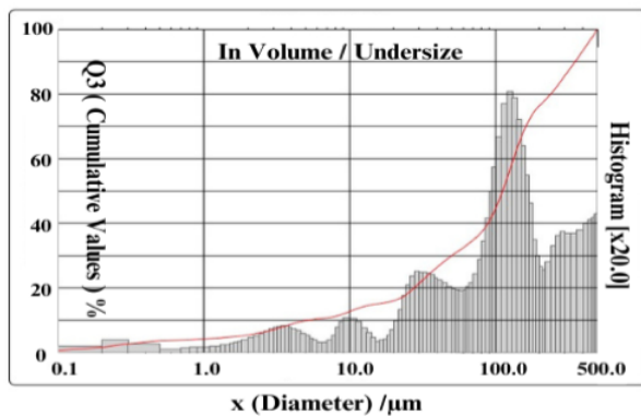
Figure 8. Particle size analyzer showing a 14% concentration with a D50:111.67 \mu\text{m}
