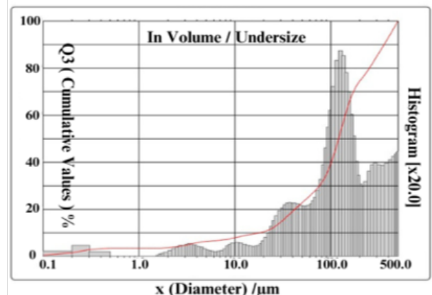
Figure 6. Particle size analyzer showing a 6% concentration with a D50:120.41 \mu\text{m}
