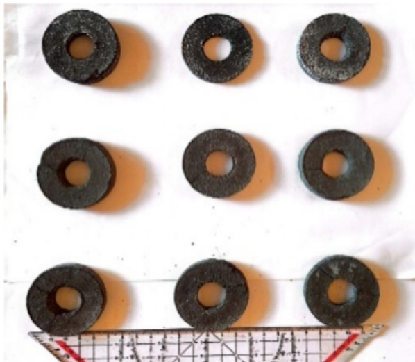
Figure 9. Sample of AMC brake pads
