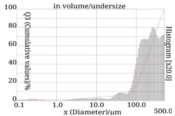
Figure 1. Graph of aluminum particle size analyzer
