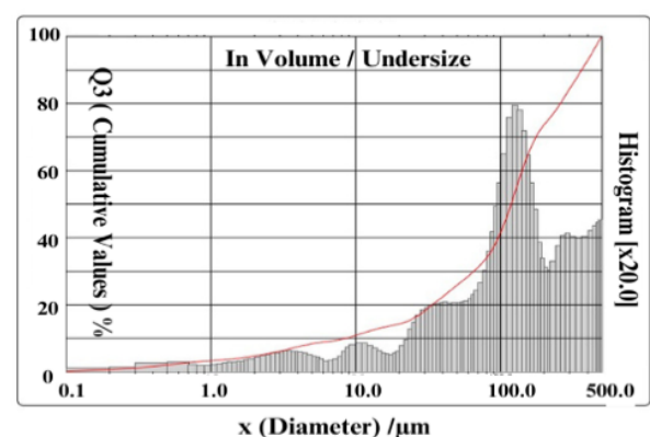
Figure 7. Particle size analyzer showing a 10% concentration with a D50:118.37 \mu\text{m}
