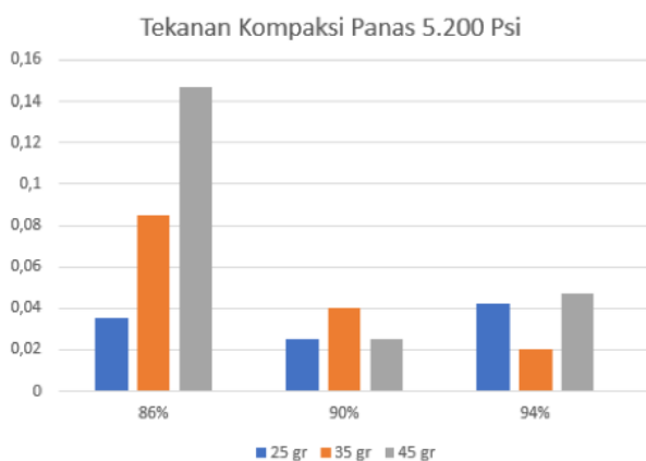
Figure 12. Graph of results from the friction coefficient test
